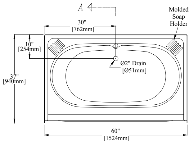
60" [1524mm] Bathtub w/ Molded Soap Holders & Removable Access Panel
